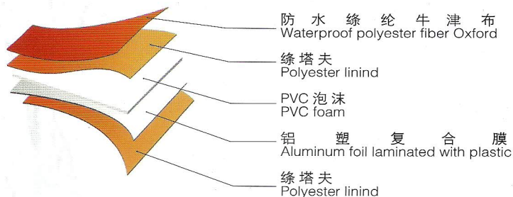
剖面图 Sectional drawing
